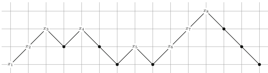
Fig. 3 The Dyck path of the DFS tree of Fig. 1
