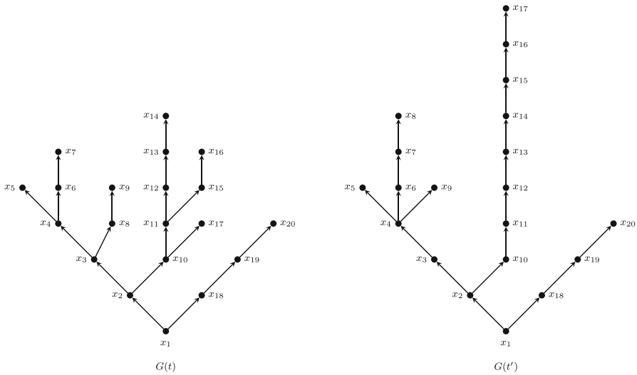
Fig. 6 DFS trees with H_{t,t'} = 6, M_{t,t'} = 3, L_{t,t'} = 2
