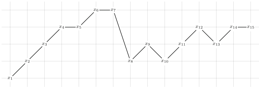
Fig. 2 The zag sequence of the DFS tree T of Fig. 4
