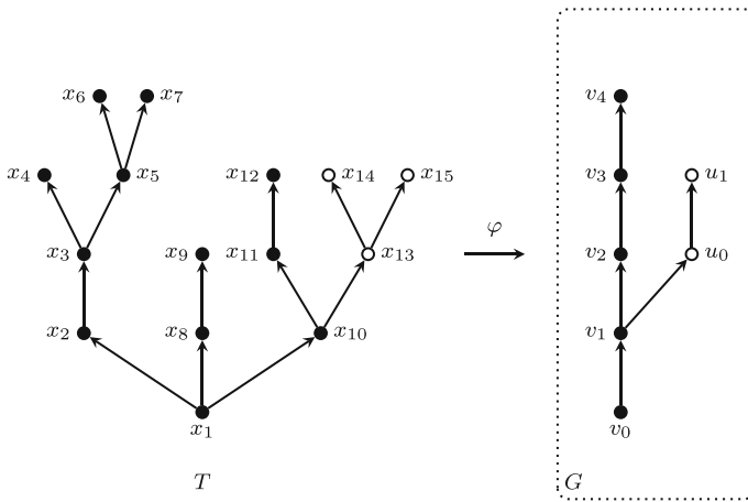
Fig. 4 Collapsing (T, x_{13}) on (W, W')
