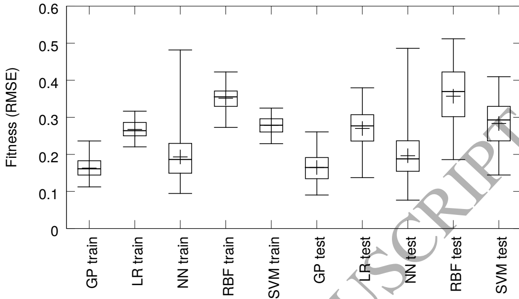
Figure 5: The results on the IS dataset (S+T) for size 10.
