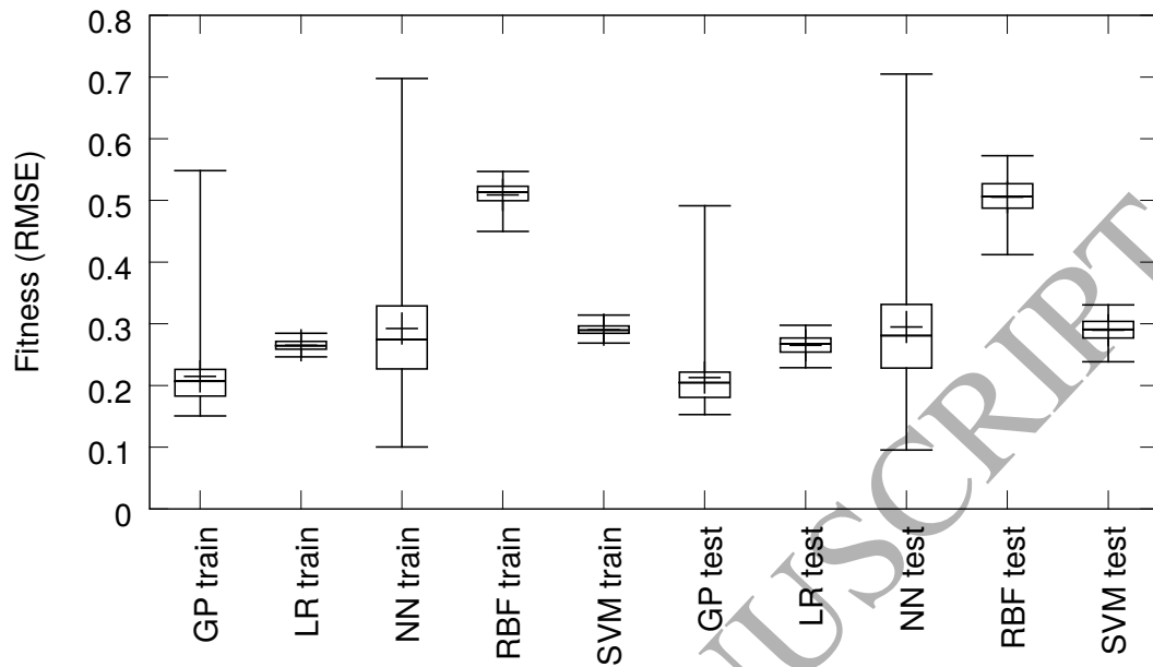
Figure 32: The results on the KS dataset (S+U+T) for size 40
