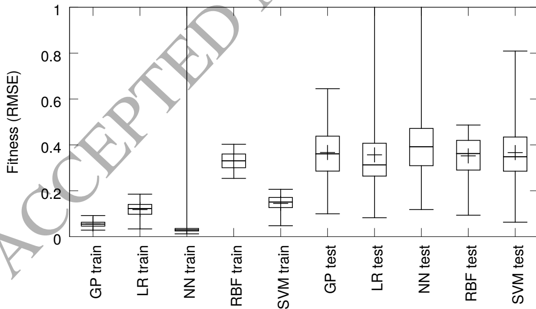
Figure 14: The results on the IS dataset (S) for size 40.
