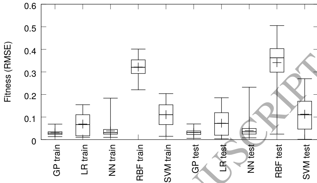
Figure 11: The results on the IS dataset (S+U) for size 30.
