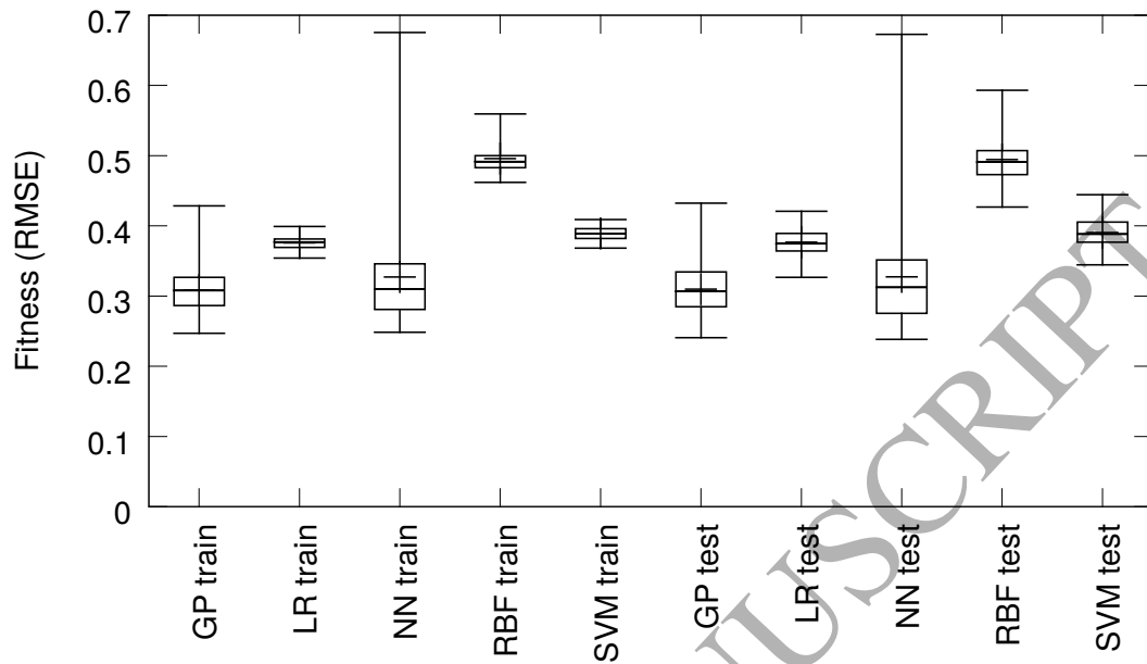
Figure 24: The results on the KS dataset (S+U+T) for size 20
