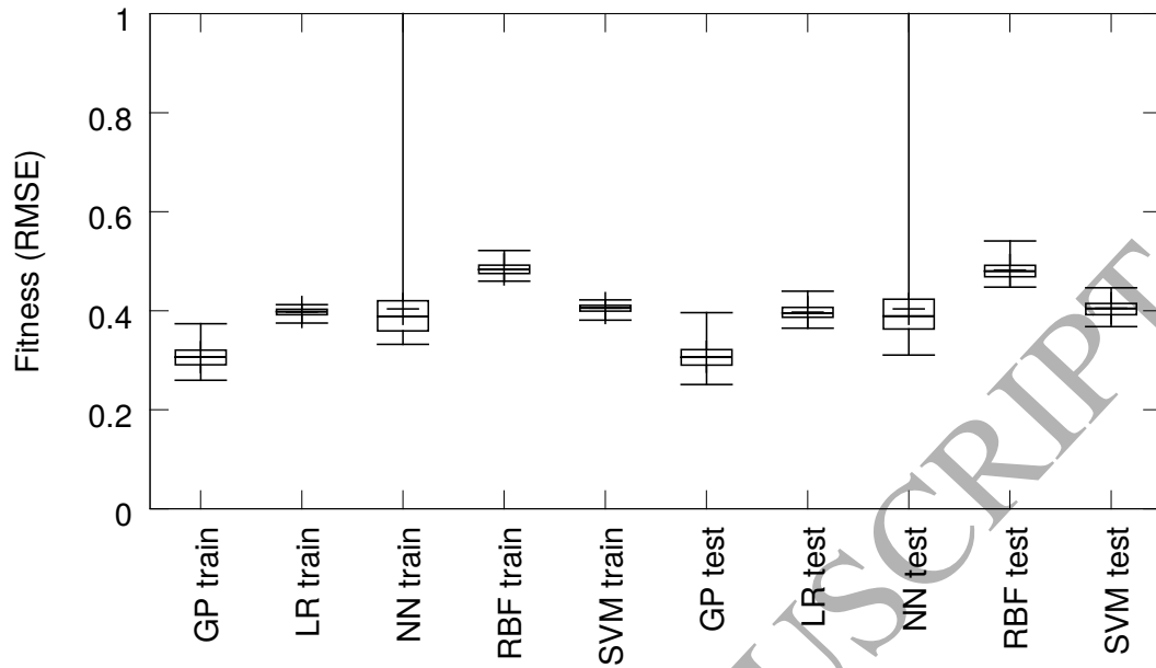
Figure 20: The results on the KS dataset (S+U+T) for size 10
