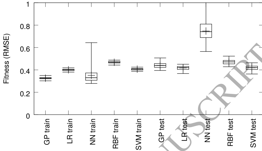
Figure 22: The results on the KS dataset (S) for size 20
