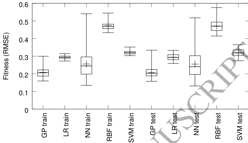
Figure 28: The results on the KS dataset (S+U+T) for size 30
