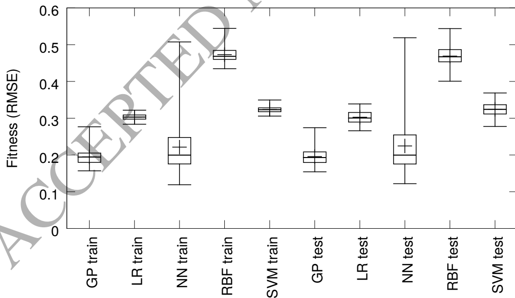
Figure 27: The results on the KS dataset (S+U) for size 30.
