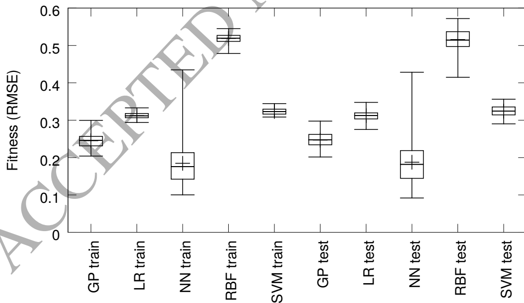
Figure 33: The results on the KS dataset (S+T) for size 40
