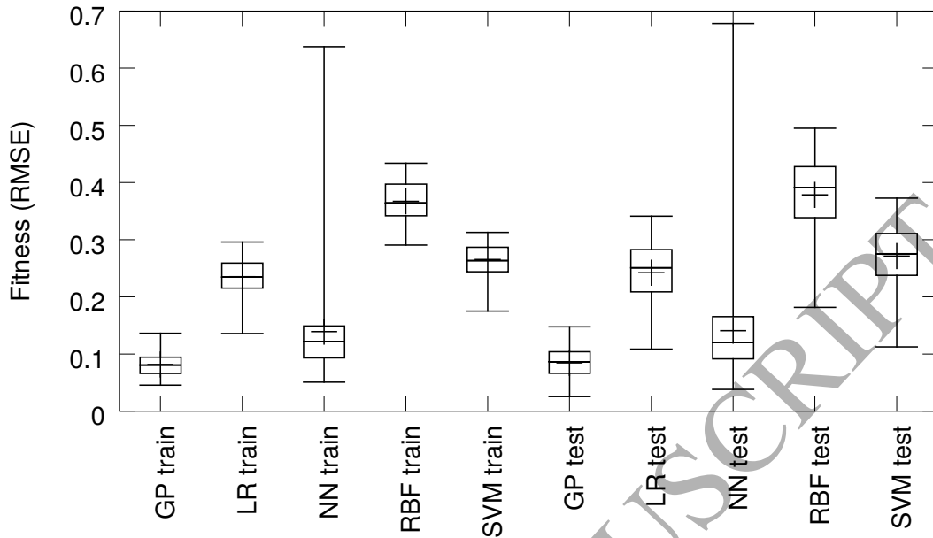
Figure 7: The results on the IS dataset (S+U) for size 20.
