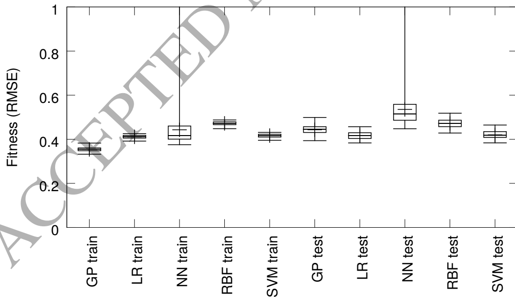
Figure 18: The results on the KS dataset (S) for size 10
