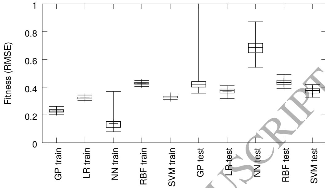
Figure 30: The results on the KS dataset (S) for size 40
