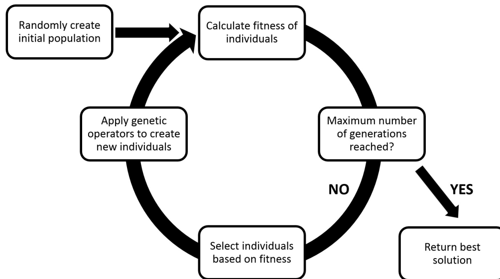
Figure 1: The GP algorithm
