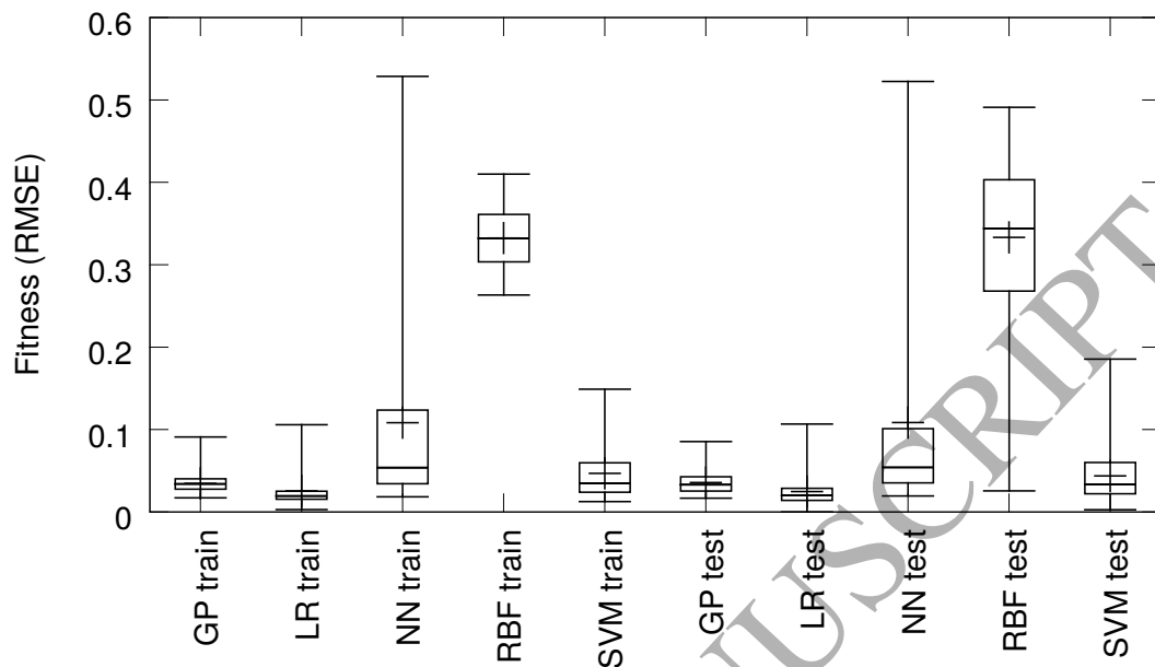
Figure 15: The results on the IS dataset (S+U) for size 40.
