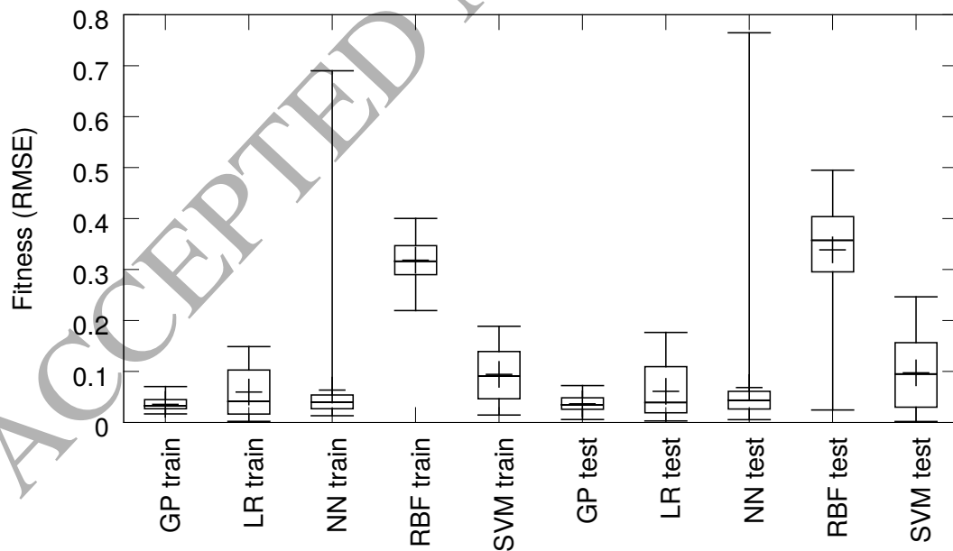
Figure 12: The results on the IS dataset (S+U+T) for size 30.
