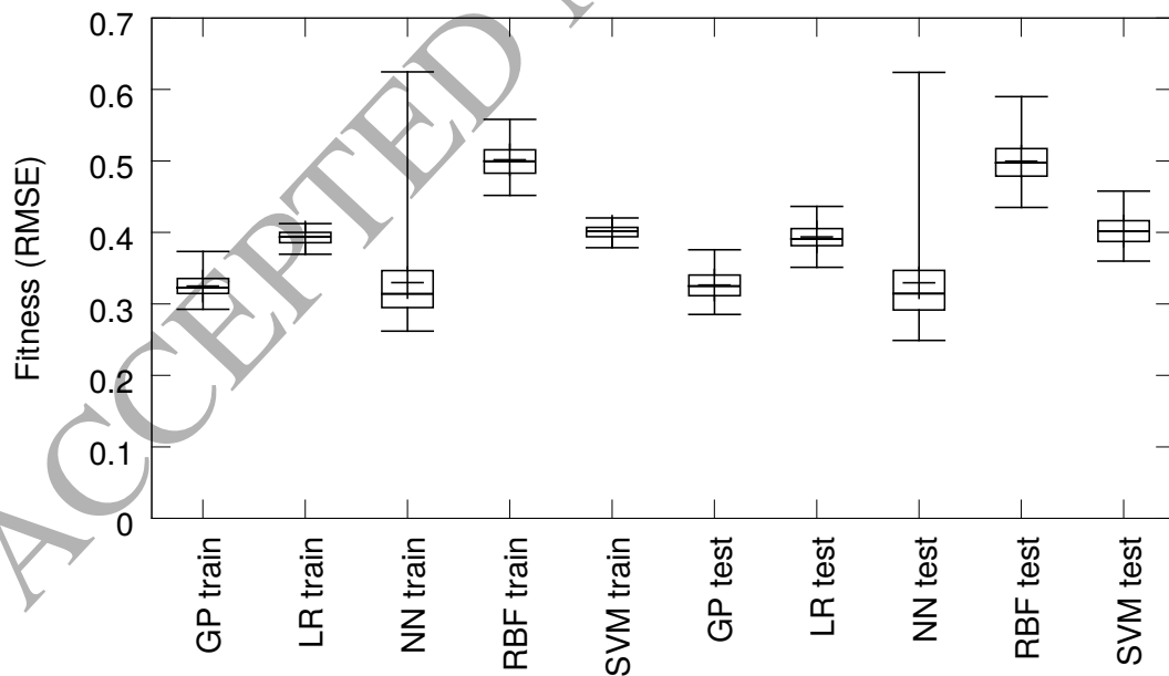
Figure 25: The results on the KS dataset (S+T) for size 20
