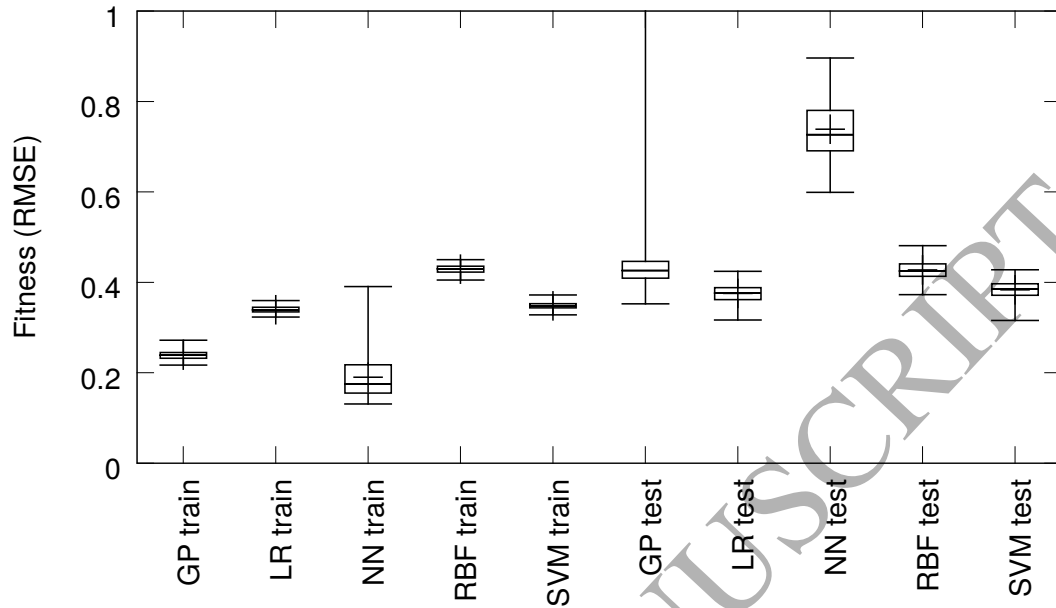
Figure 26: The results on the KS dataset (S) for size 30
