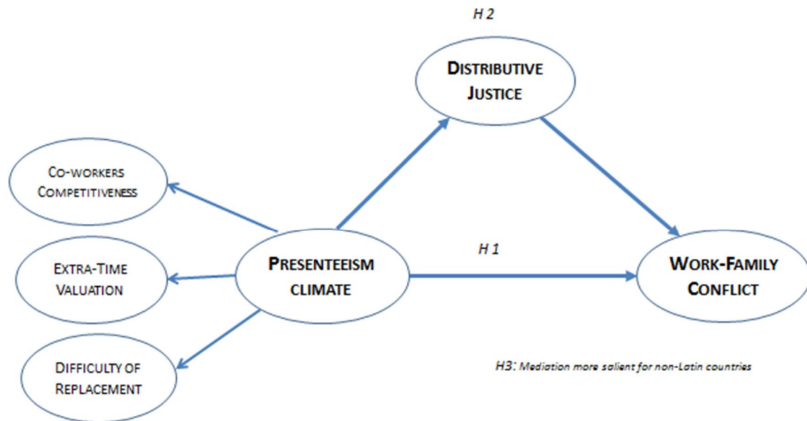
Figure 1. Conceptual Framework: Mediation Analysis
