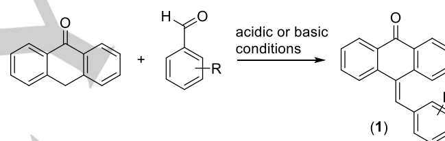
Scheme 1. Synthesis of 10-substituted benzylidene anthrones ( 1 ).
