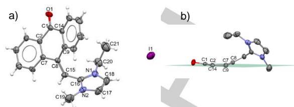
Figure 1. a) MERCURY diagram of compound 4 , using 30% probability level ellipsoids; b) the asymmetric boat conformation of the central ring in the anthrone unit. Hydrogen atoms and the outer aromatic rings are omitted for clarity
