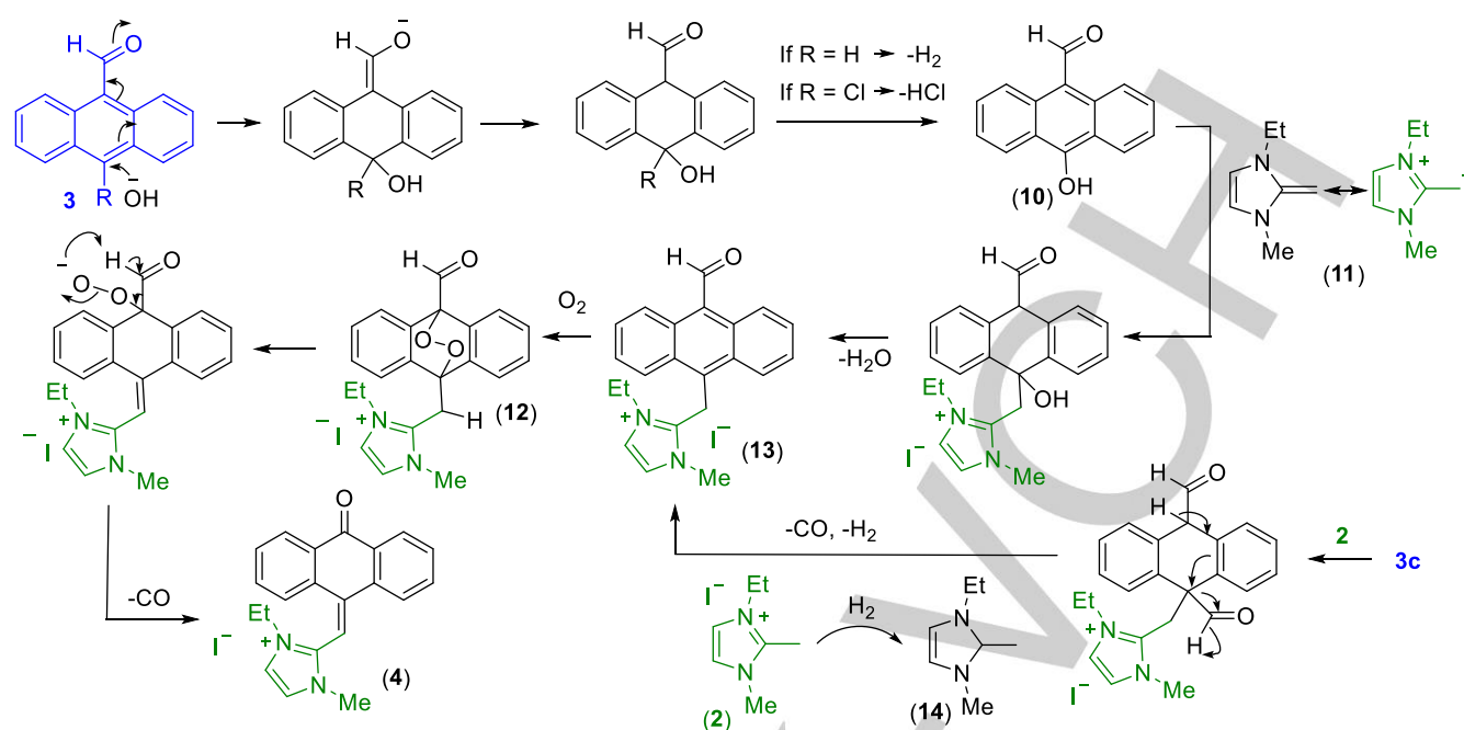
Scheme 3. Proposed mechanism for the formation of 4 .
