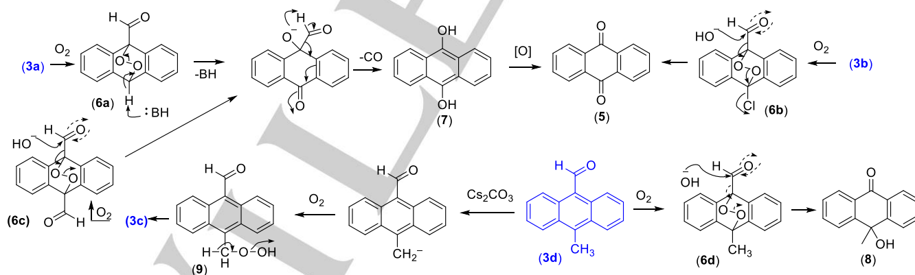
Scheme 2. Proposed mechanism for the formation of 5 and 8 .
