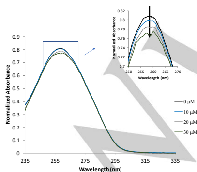
Figure 2. Absorption spectra of CT-DNA (15 \mu\text{M} ) in the presence of increasing concentrations of compound 4 (0–30 \mu\text{M} ). Inset: maximum absorbance peak hypochromism due to the increase of compound 4 concentrations – indicated by the black arrow.
