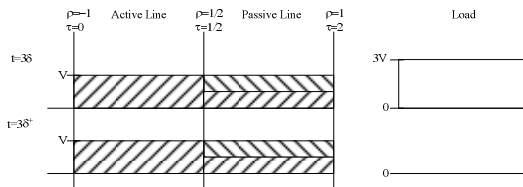
Fig. 6. Propagation voltage waves and load voltage between 3\delta < t < 3\delta
