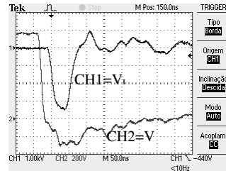
Fig. 8. Experimental negative pulse, V_L , 1kV/div and input charging voltage V , 200V/div, both width 50 ns/div
