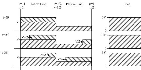
Fig. 5. Propagation voltage waves and load voltage between 2\delta < t < 3\delta
