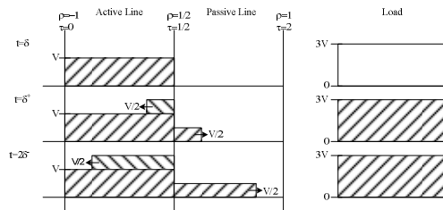
Fig. 4. Propagation voltage waves and load voltage between \delta < t < 2\delta
